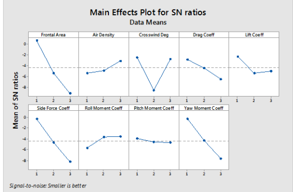
Figure51: Taguchi SNR plot for Aerodynamic properties
