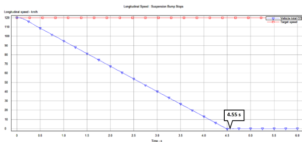
Figure26: Brake Speed km/h-Time(s) "MAFSMC_ON"
