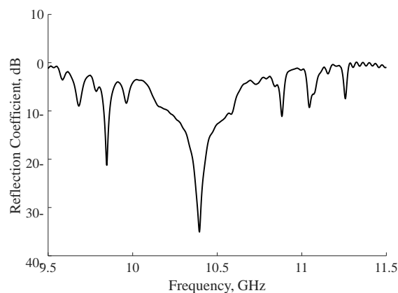
Figure 11: Reflection coefficient of the phased array antenna when the main lobe is at 15.7^\circ .
