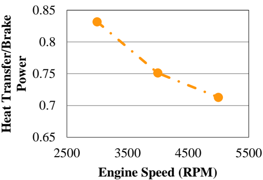
Figure 9: Experimental Heat Transfer to Brake Power Ratio
