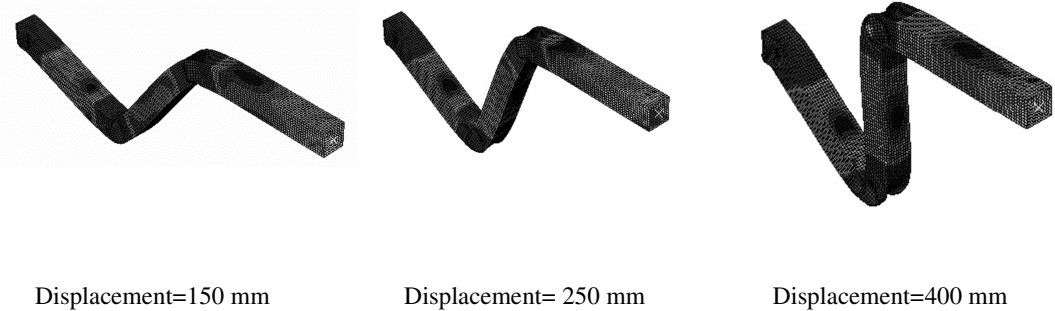
Fig12. shape of deformation of the S-rail with geometries of R=550\text{ mm} , q=25 , W=50\text{ mm} and t=2\text{ mm} at end displacement of 150, 250 and 400 mm.
