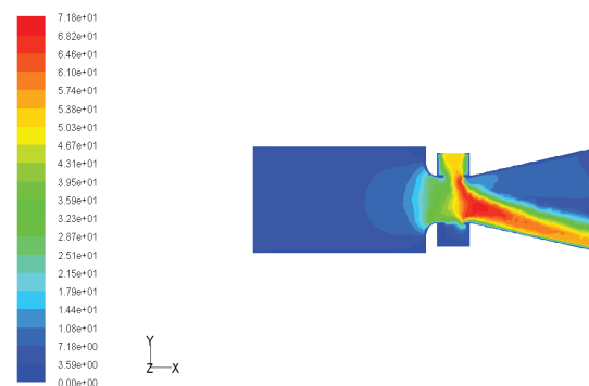
Fig. 10. Velocity distribution contour in the optimum venturi
