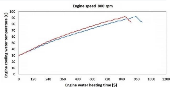
Figure 10: Comparison of temperature changes in the electric water pump with 800 rpm compared to the normal state
