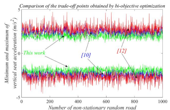
Figure 6. Minimum and maximum points of vertical seat acceleration resulted by C_1 [this work], C'_1 [10] and C''_1 [12] for the 5-degree of freedom vehicle model exited by 1000 different non-stationary random roads.
