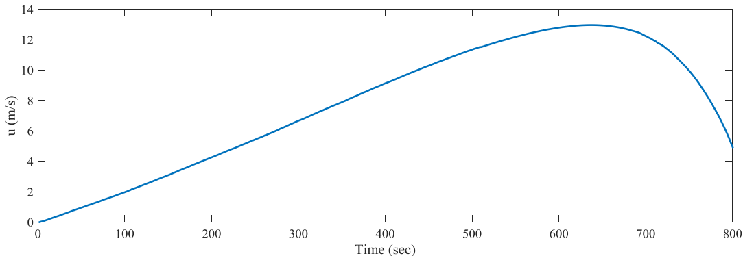
Fig18. longitudinal velocity of the vehicle
