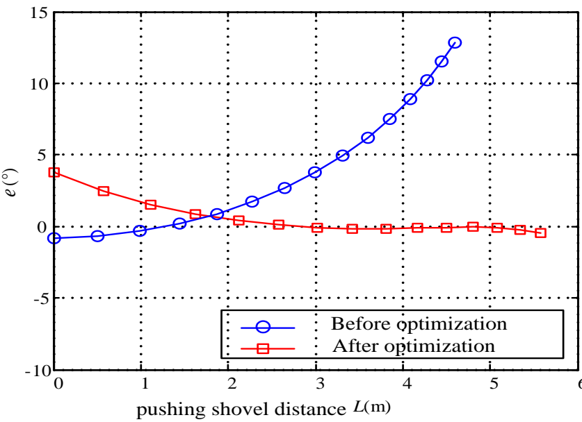
Fig6. Before and after optimization in the process of horizontal push shovel
