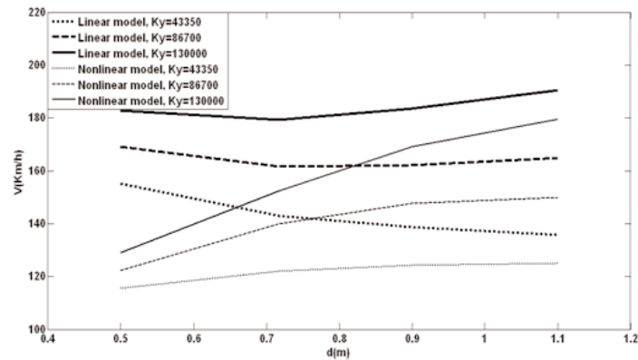
Fig. 5. Influence of the track gauge on the hunting behavior
